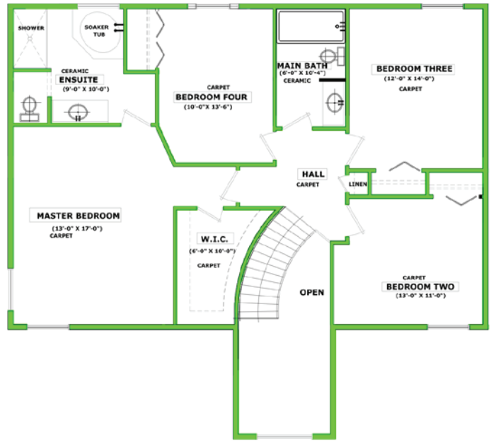
Second Floor Plan–1,121 Sq. Ft.
