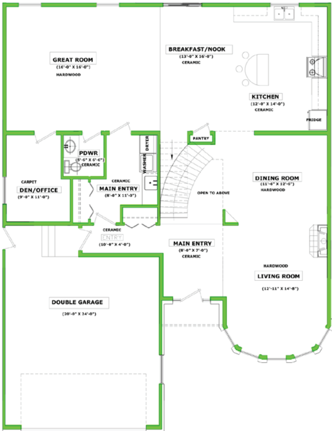
Ground Floor Plan– 1,467 Sq. Ft.
